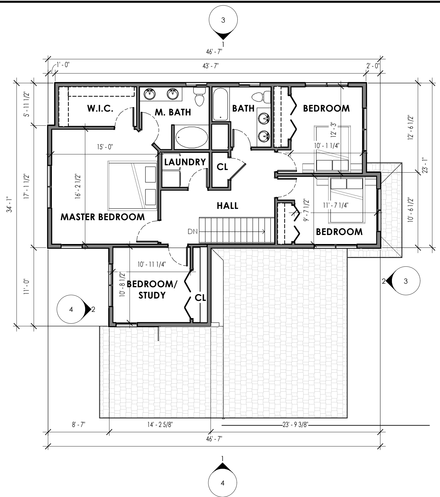
2 SECOND FLOOR (EXTRA BEDROOM OPTION) 1/8" = 1'-0"
