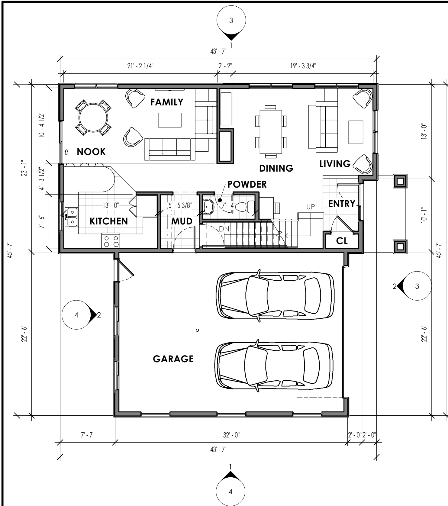
1 FIRST FLOOR (EXTRA BEDROOM OPTION) 1/8" = 1'-0"
